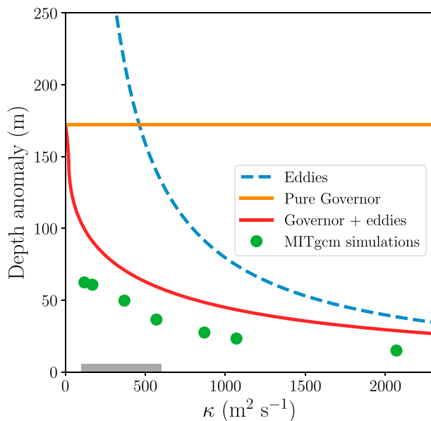
Figure 7. Isopycnal depth anomaly from a series of Arctic simulations. The green circles represent the results from an ensemble of MITgcm simulations in which \kappa_{GM} has been varied, while the lines represent the theoretical predictions. The solid red line represents the three-way balance prediction, the solid orange line is the pure Ice-Ocean Governor prediction ( \kappa = 0 \text{ m}^2/\text{s} ), and the dashed blue line represents the predicted solution for an eddy equilibrated gyre in the absence of the Ice-Ocean Governor. The surface stress for the dashed blue line has been calculated using the ensemble average ice-ocean relative velocity in equation (3). The gray shaded region on the x axis highlights the estimated range of 100–600 \text{m}^2/\text{s} for eddy diffusivity in the BG (Meneghello et al., 2017).
