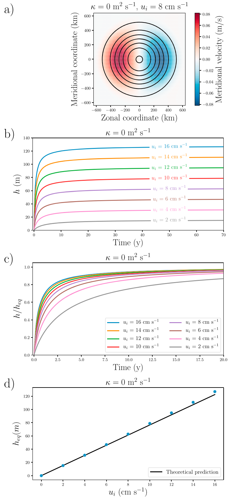
Figure 4. (a) Eulerian-mean meridional velocity (colors) and layer thickness (contours, with a contour interval of 10 m) from the final 10 years of the \kappa = 0 \text{ m}^2 \text{ s}^{-1} , u_i = 8 \text{ cm/s} simulation. (b) Temporal evolution of the isopycnal depth anomaly for a range of imposed ice velocities with the thickness diffusivity, \kappa , set to 0. (c) The normalized isopycnal depth anomaly shows that the adjustment timescale depends on u_i . (d) Equilibrium isopycnal depth anomaly plotted against u_i (dots), with the prediction from equation (7) using the values from Table 1 and \alpha = 1 shown by the black line.
