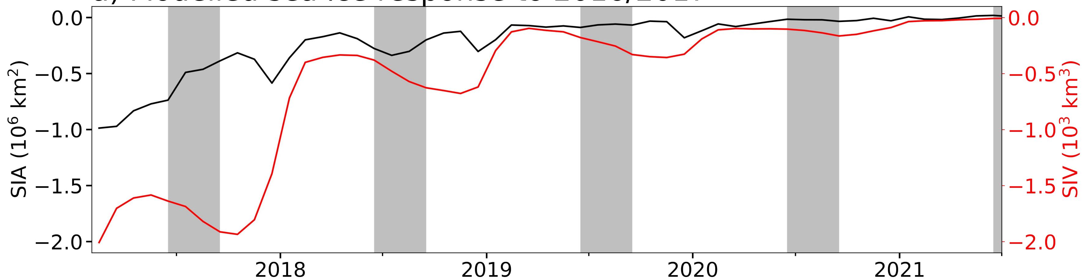
b) Linear temperature response to 2016/2017
